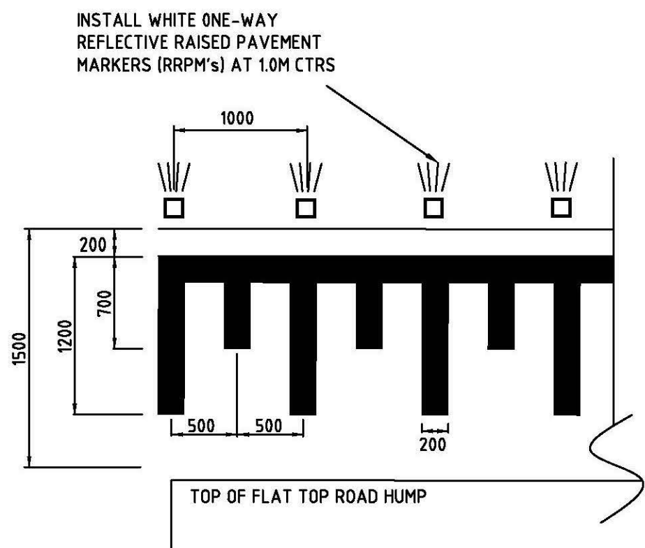
PAVEMENT MARKINGS AND R.R.P.M'S FOR ROAD HUMPS NOT TO SCALE
